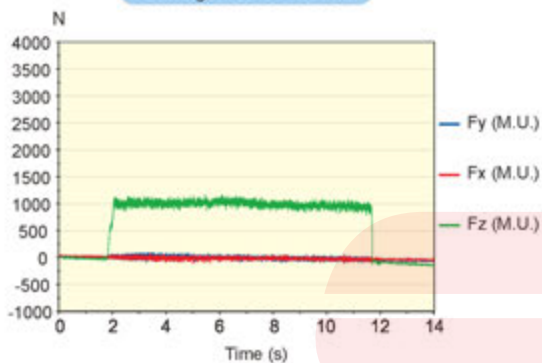
Cutting force of 1588SL
