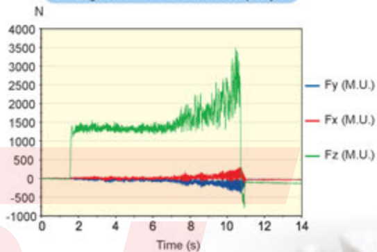
Cutting force of Product of company A
