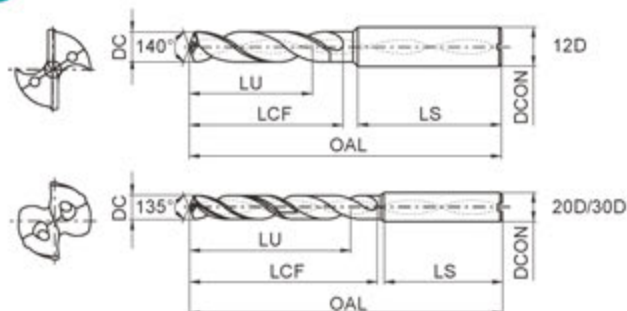
Straight shank
